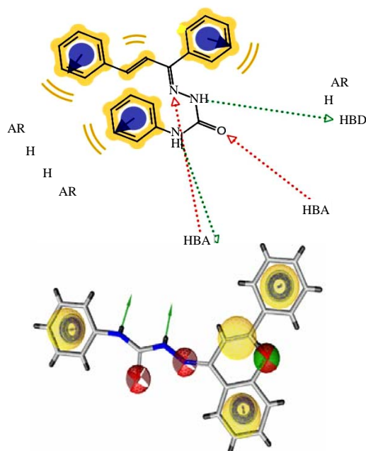
Fig. 1: Pharmacophore of the designed chalconesemicarbazone by ligandsout 2.02
