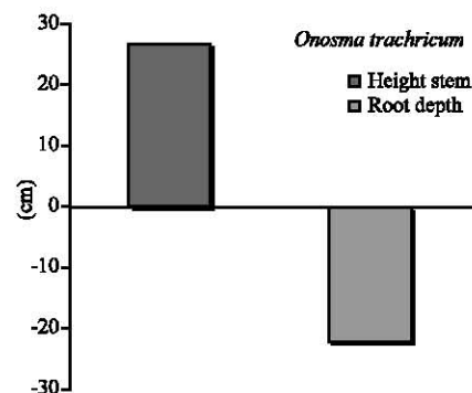
Fig. 3: Onosma trachtricum average root depth and stem height
