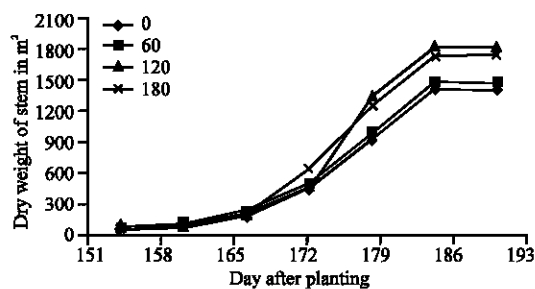
Fig. 7: Effect of nitrogen fertilizer rates on dry weight of stem m -2 during the season
