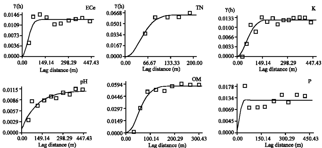
Fig. 2: Omnidirectional semivariogram for soil parameters
