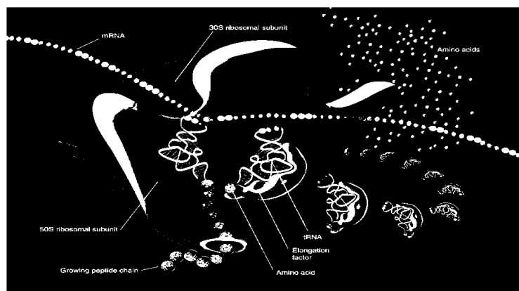
Fig. 2: Mechanism of inhibition of the protein synthesis
