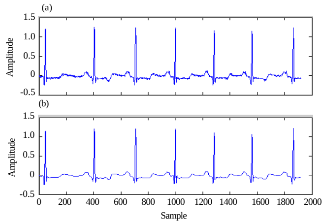
Fig. 4: De-noised ECG signal (with Bior3.9); a) Original signal with noise; b) De-noised signal
