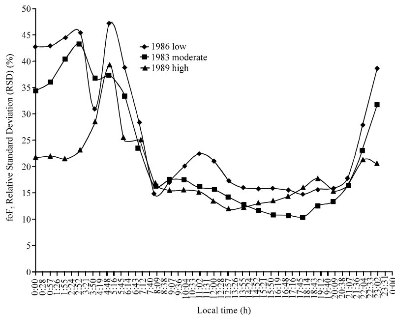
Fig. 14: Variations of the critical frequency of the F_2 layer using Relative Standard Deviation (RSD) averaged over the whole year for low, moderate and high solar activity for Dakar
