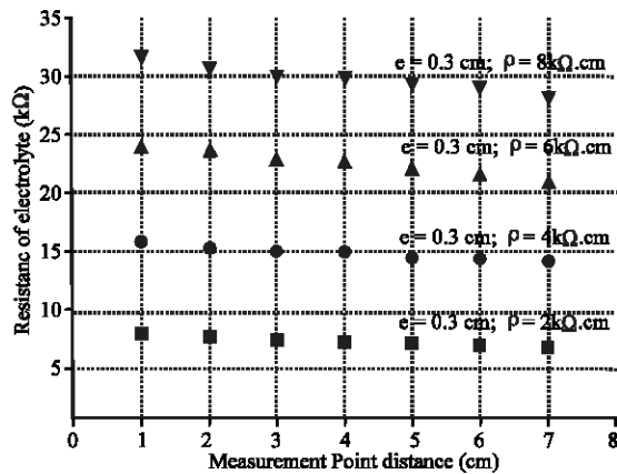
Fig. 4: The electrolytic resistance according to distance
