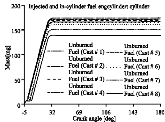
Fig. 3: Unburned fuel 2 holes
