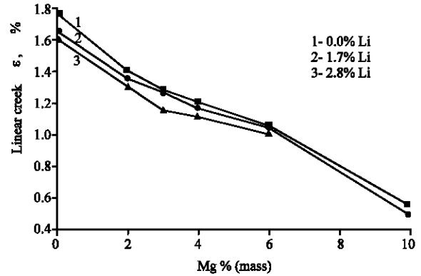
Fig. 1: Linear creek of alloys Al-Li-Mg
