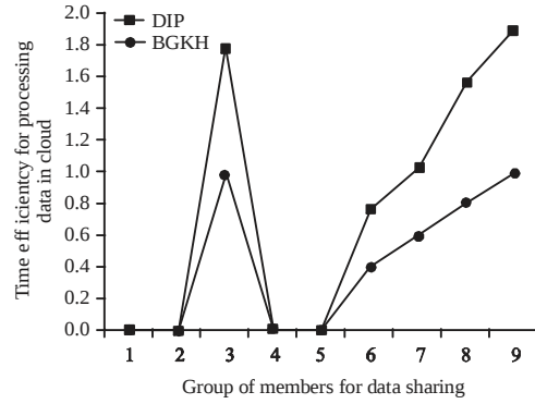
Fig. 6: Computational time efficiency in application process of DIP and proposed Schema in access control in usability
