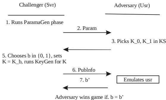
Fig. 4: The attacker activity for BGKM’s key concealing residence. With the information of PubInfo, the attacker is not able to distinguish one of its selected important factors from the other
