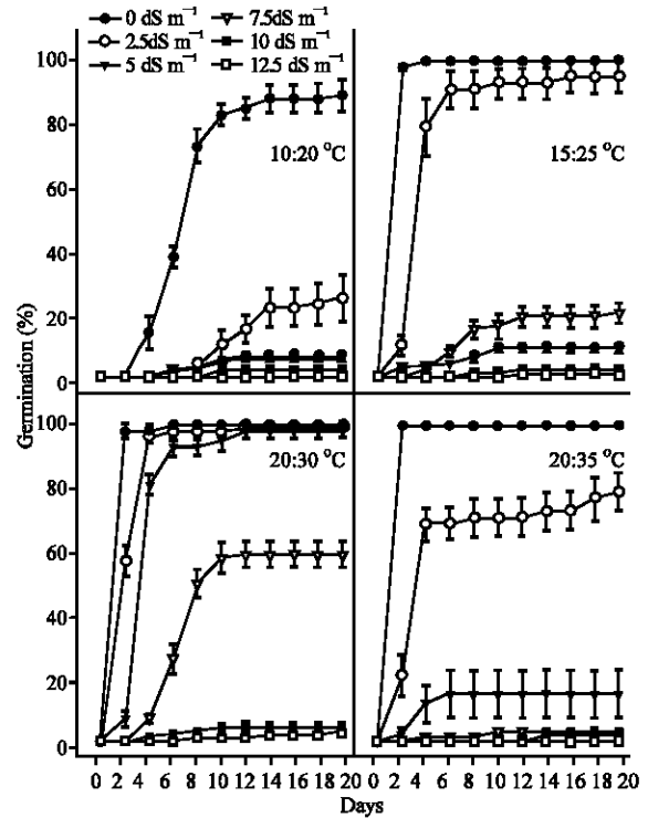
Fig. 2: Cumulative mean percent germination of dill ( Anethum graveolens ) seeds over time in 0, 2.5, 5, 7.5, 10 and 12.5 dS m -1 NaCl in 12 h light : 12h dark photoperiod. Bars represent mean \pm SE
