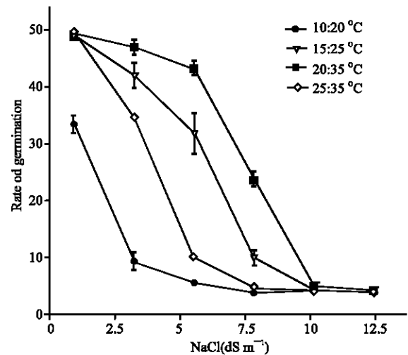
Fig. 3: Rate of germination of dill ( Anethum graveolens ) seeds under various salinity and thermoperiod treatments as represent mean \pm SE
