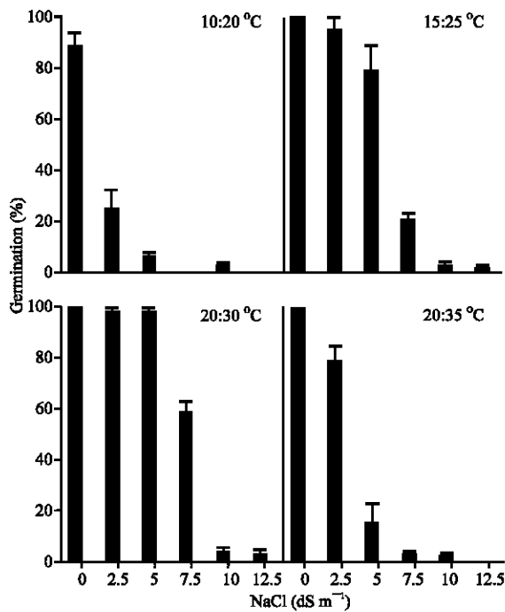
Fig. 1: Mean final percent germination of dill ( Anethum graveolens ) in various salinity and temperature conditions. Bars represent mean \pm SE
