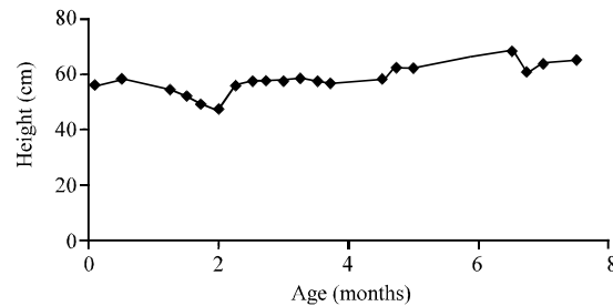
Fig. 3: Height variation with age of children
