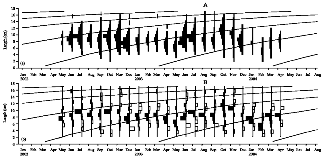
Fig. 3: Length-Frequency for Macrobrachium vollenhovenii with growth curve super imposed (A) Original and (B) Restructured
