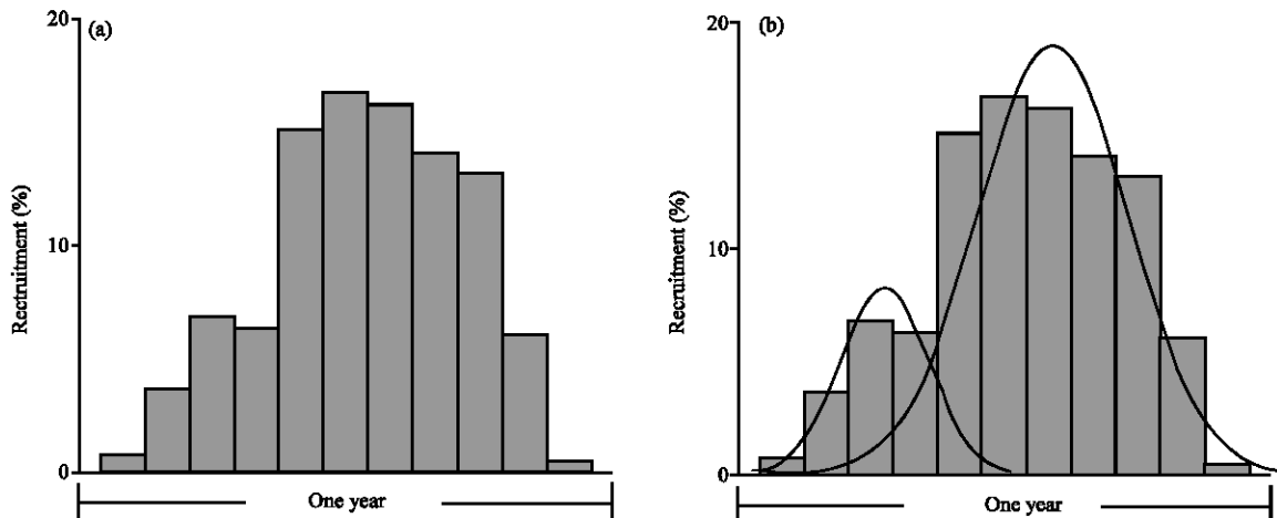
Fig. 5: (A) Backward projection, along a trajectory defined by the VBGF, of the restructured length frequency data onto an arbitrary one-year timescale for M. vollohovenii . The months on the X axis cannot be located exactly (hence the abscissa is an arbitrary year) because of the location parameter ( t_0 ) of the VBGF. (B). Recruitment pattern decomposed into pulses exhibiting two peaks of unequal pulse strength for M. vollohovenii . The pattern was decomposed using NORMSEP and fitted with two Gaussian distributions
