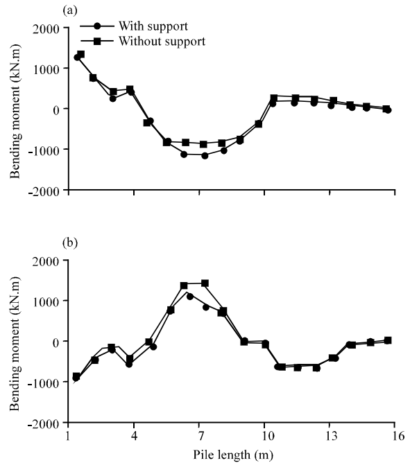
Fig. 4: Comparing diagram of bending moment between with and without support
