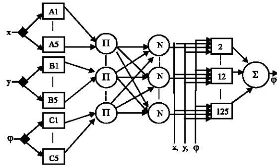
Fig. 2: ANFIS architecture
