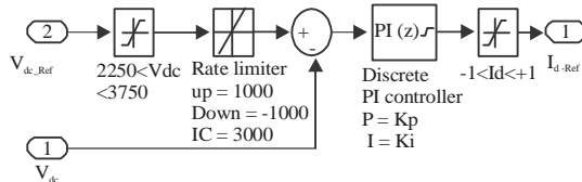
Fig. 6: DC bus voltage regulator
