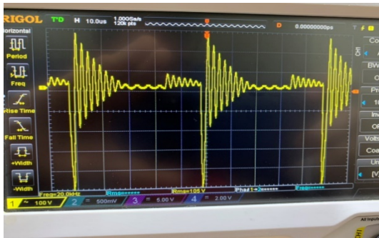
Fig. 7: The output voltage from transformer
