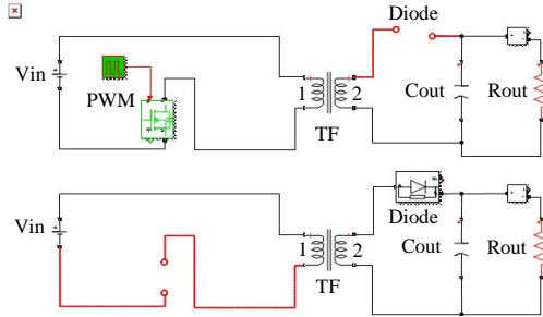
Fig. 2: Operated flyback
