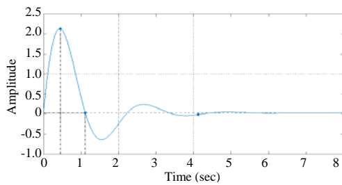
Fig. 9: Step response
