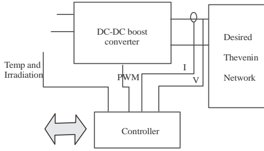
Fig. 1: Solar PV system
