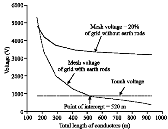
Fig. 5: Determination of the total required length using the safety parameter curves assuming a layered soil of top and bottom layers of 400 and 600 \Omega\text{m} , respectively
