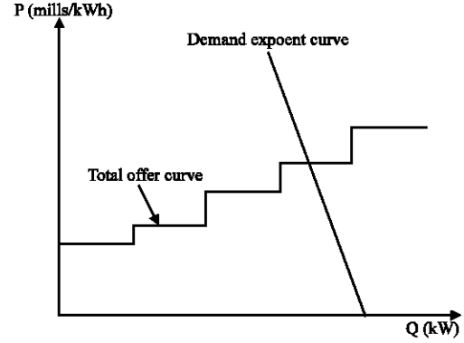
Fig. 3: Typical total offer and demand exponent curves
