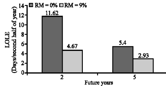
Fig. 8: LOLE values for second study using MCS
