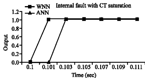
Fig. 9d: Trip output for internal fault with CT saturation
