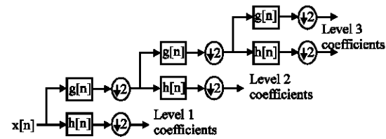
Fig. 3: Block diagram of filter analysis
