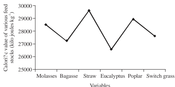
Fig. 4: Calorific value of various feed stocks
