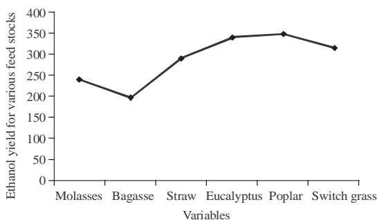
Fig. 2: Ethanol yield for various feed stocks
