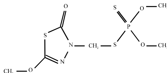
Fig. 1: Methidathion formula (Kim et al. , 2011)
