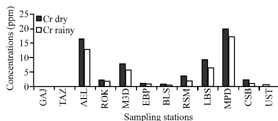
Fig. 2: Seasonal variations in concentrations of Cr with sampling stations
