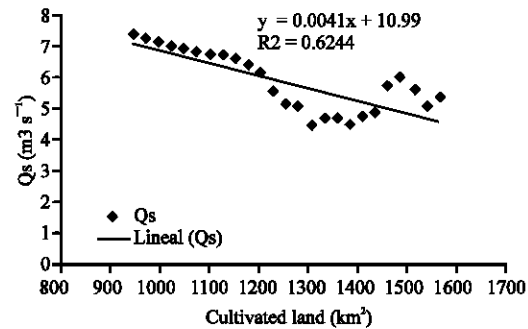
Fig. 9: Linear regression between spring discharge ( Q_s ) and cultivated land
