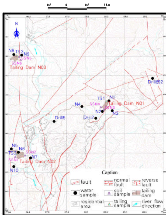
Fig. 2: Makeng underground iron mine's tailing storage facilities map
