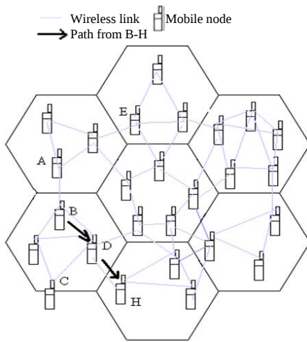
Fig. 2: A Mobile ad hoc wireless network
