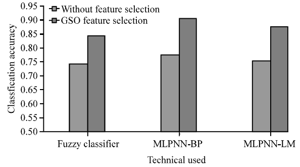
Fig. 2: Classification accuracy for GSO feature selection
