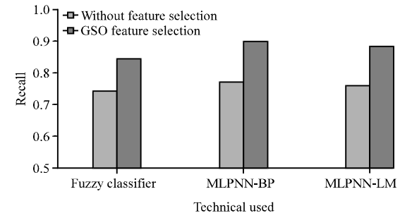
Fig. 4: Recall for GSO feature selection
