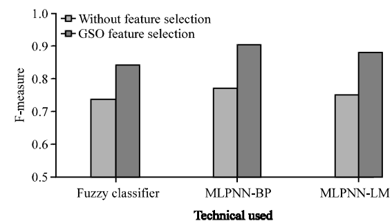
Fig. 5: F-measure for GSO feature selection
