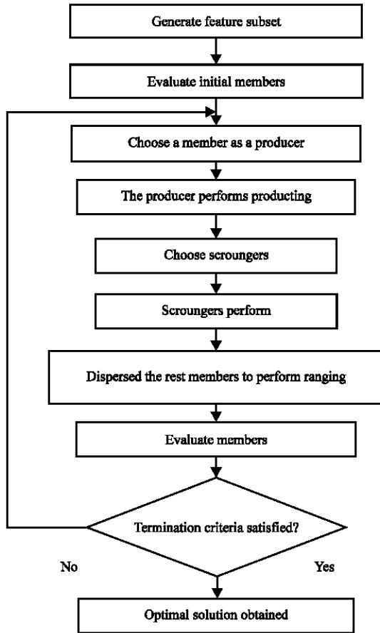
Fig. 1: Flowchart for proposed methodology feature subset
