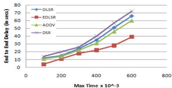
Fig. 6: End to End Delay Comparison between EOLSR and other Protocols
