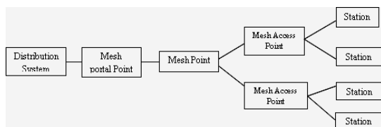
Fig. 1: IEEE 802.11s wireless mesh network architecture
