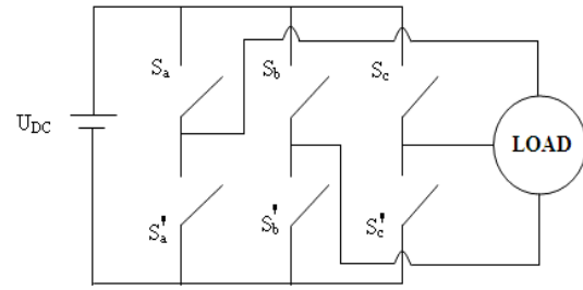
Fig. 5: Circuit of voltage source inverter
