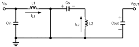
Fig. 3: SEPIC converter current flow during Q1 on-time
