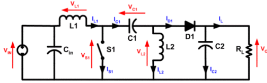
Fig. 2: SEPIC converter
