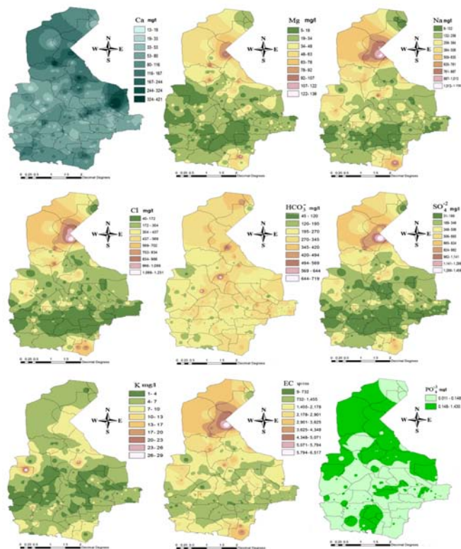
Fig. 4: The scatter of anions and cations in Sistan and Baluchistan ground water resources
