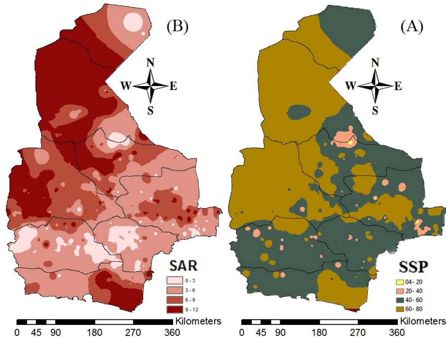
Fig. 5: a) The Scatter of SSP index and b) the scatter of SAR index
