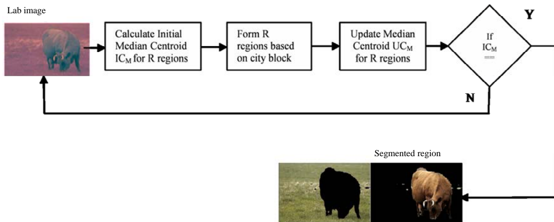
Fig. 4: Region clustering
