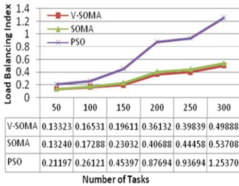
Fig. 3: Average of load balancing using 20VM
