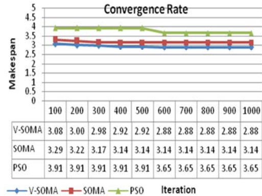
Fig. 5: Convergence analysis
