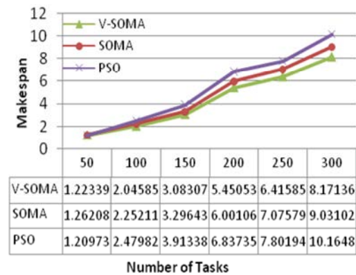
Fig. 1: Average makespan using 20VM
