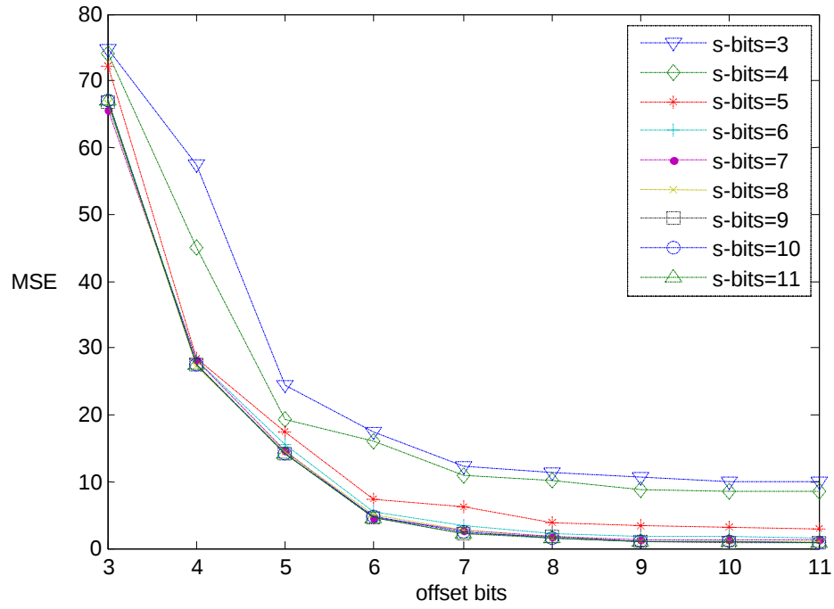
Fig. 3: MSE vs quantization parameters for lena 256×256
