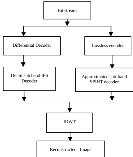
Fig. 7: Block diagram for proposed decoder
