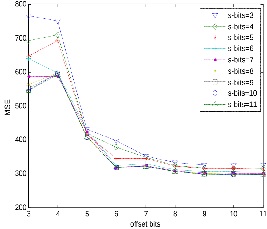
Fig. 5: MSE vs. quantization parameters for Boat 512×512
