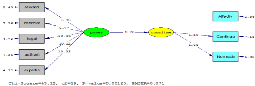
Fig. 4: Significance figures of total research
