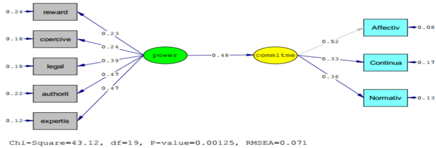
Fig 3: Results of coefficients and standard estimation of research general model
