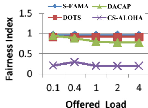
Fig. 10: Jain's fairness index for the four protocols
