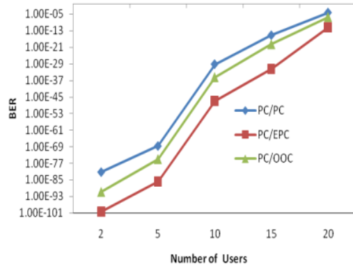
Fig. 5: Comparison of BER with varied number of users
