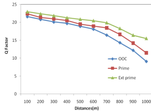
Fig. 7: Comparison of Q-factor for various coding schemes without applying distance based power allocation algorithms
