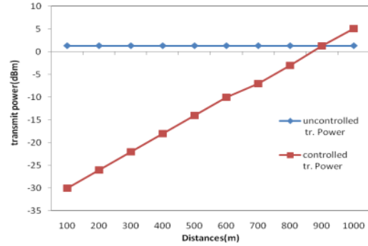
Fig. 9: Comparison in terms of transmission power between conventional scheme of transmission and new design with dista
