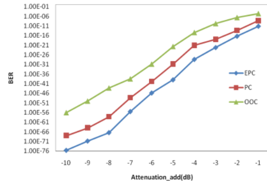
Fig. 3: Variation in BER with change in attenuation
