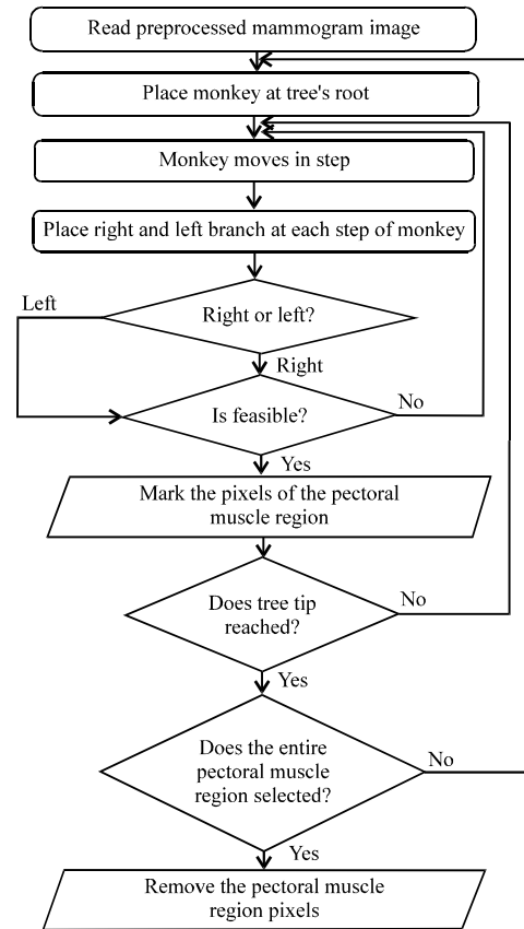
Fig. 1: Flowchart for removing pectoral muscle region using MSO
