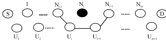
Fig. 2: Enhanced triple umpiring system model; N_{i-1} , N_i , N_{i+1} , ..., N_m intermediate nodes in the active path. U_1 , U_{i+1} , ..., U_{m+1} = Corresponding umpires. For node N_{i-1} , U_1 , U_{i+1} in the forward path and N_{i+1} , U_i , U_{i+1} in the reverse path. Assume that node N_i becomes culprit node in the packet forwarding operation. ETUS form an new route using umpiring nodes. Node N_{i-1} , U_i and U_{i+1} used to form an alternative path to reach node N_{i+1} . In the alternative path, there is no independent umpires are used (i.e.) self-umpire. Self-umpire nodes have dual roles packet forwarding and umpiring
