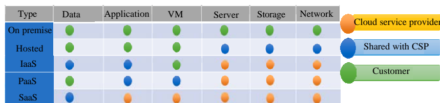
Fig. 2: Segregation of control between customer, CSP and shared model
