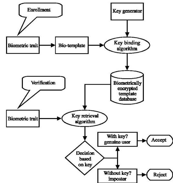
Fig. 15: Data flow diagram of key based BE
