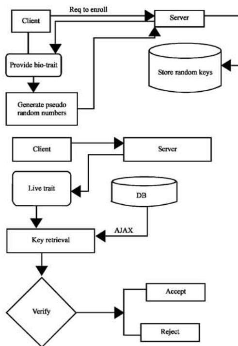
Fig. 16: AJAX technology in biometric security
