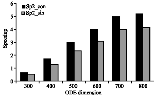
Fig. 5: Speedup of ODE with initial condition in constant and sinusoid form on eight processors
