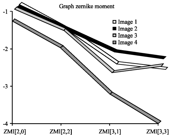
Fig. 6: Features of digit 0 extracted using Zernike invariants
