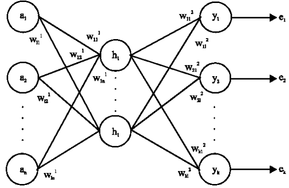
Fig. 2: Back-propagation architecture
