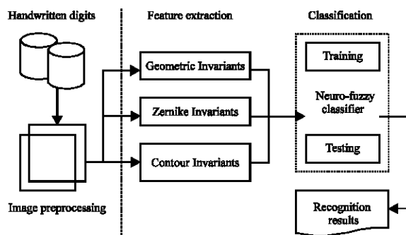
Fig. 1: A framework of neuro fuzzy classifier for handwritten digits recognition
