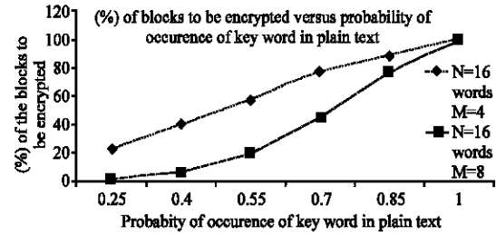
Fig. 2: Variation of r with \alpha [Note: the results are given only for N=16 as because if N is high, the computation using binomial formula becomes unmanageable. In that study, Laplace approximation has to be used]
