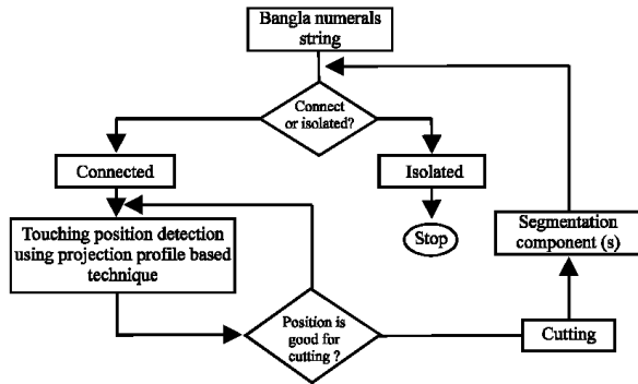
Fig. 2: Segmentation scheme
