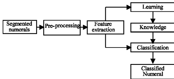
Fig. 3: Numeral recognition
