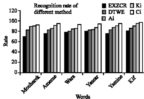
Fig. 6a: Recognition rate for the six command words using different methods.
