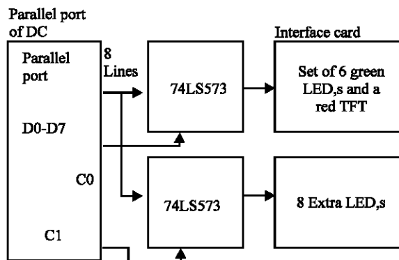
Fig. 4: Parallel port interface
