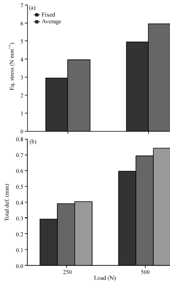
Fig. 6: Stress and deformations results
